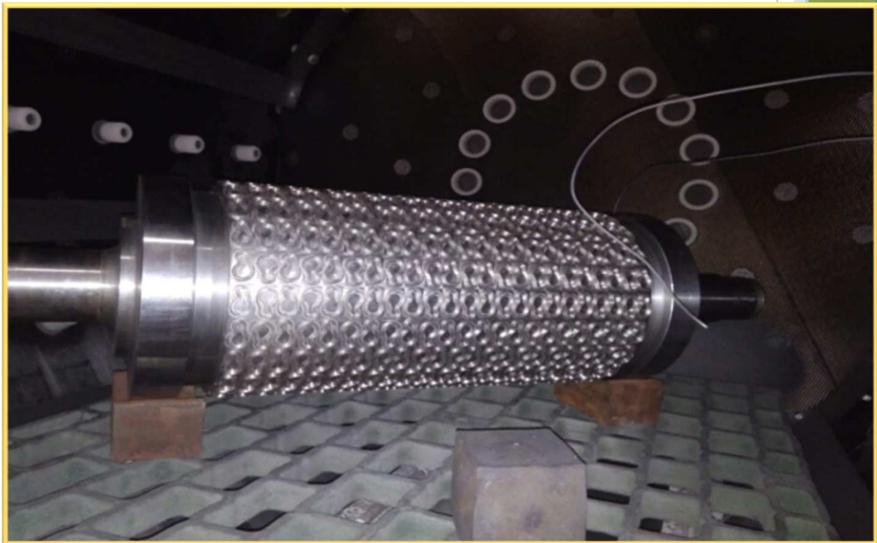
Roller Die during Vacuum Heat Treatment
